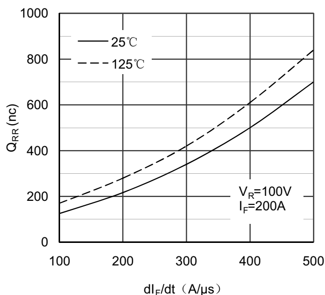
Figure 2. Reverse Recovery Charge vs dI_F/dt
