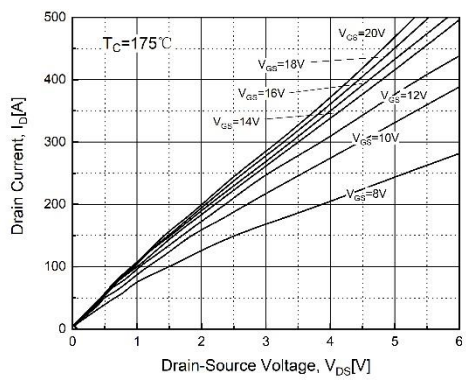
Fig. 2. Typical Output Characteristics @ 175^{\circ}\text{C}
