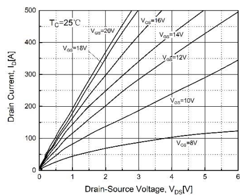
Fig. 1. Typical Output Characteristics @ 25^{\circ}\text{C}
