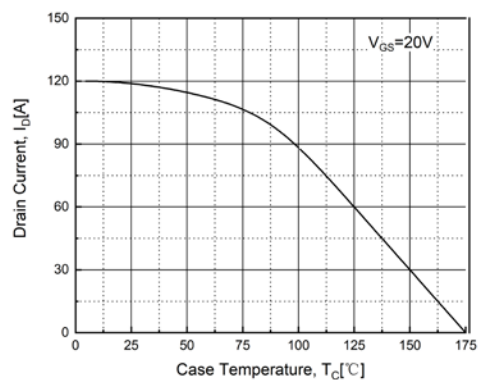
Fig. 12. Maximum Drain Current vs. Temperature
