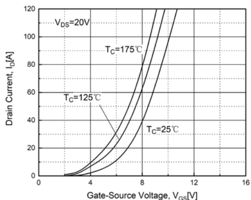
Fig. 7. Transfer Characteristics
