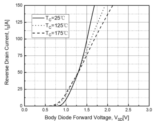
Fig. 6. Diode Forward Characteristics
