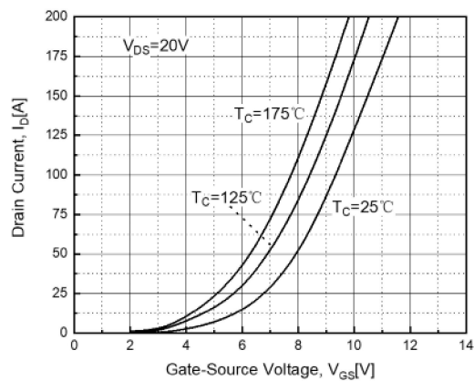
Fig. 5. Transfer Characteristics
