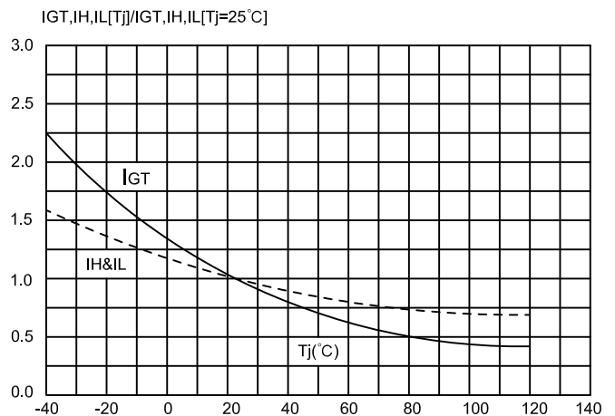
Fig.6: Relative variations of gate trigger current, holding current and latching current versus unjunction temperature
