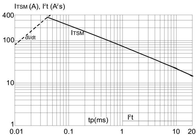
Fig.5: Non-repetitive surge peak on-state current for a sinusoidal pulse with width t_p < 20\text{ms} and corresponding value of I^2 t ( dI/dt < 10\text{A}/\mu\text{s} )
