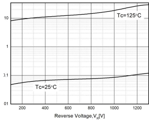
Fig. 2. Typical Characteristics: V_R vs. I_R
