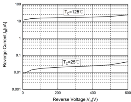
Fig. 2. Typical Characteristics: V_R vs. I_R
