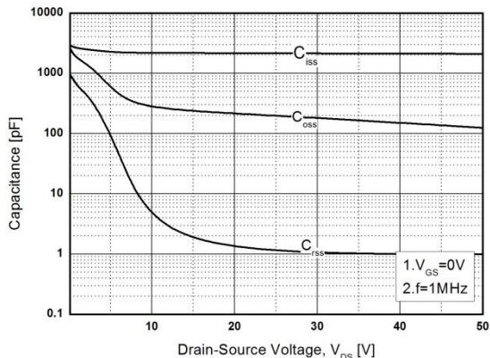
Fig. 5. Capacitance Characteristics
